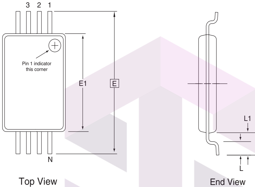
COMMON DIMENSIONS (Unit of Measure = mm)
